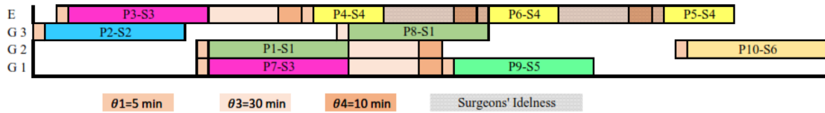
FIGURE 2. The resource graph based on the proposed schedule for the sample day (Total Surgeons' Idle time = 90)
