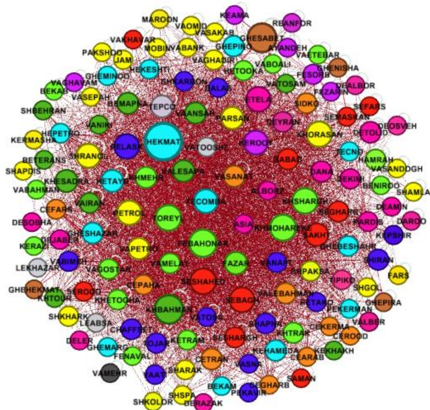
Fig. 8. The network visualization with 0.082 modularity and 12 communities
