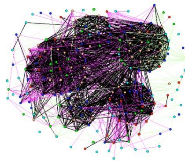
Fig. 2. Investors network (Tomminello et al., 2012)
