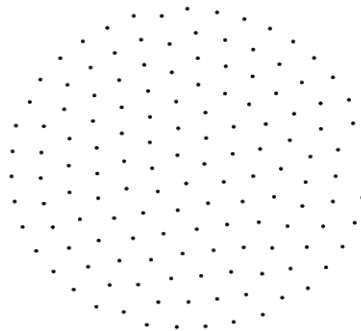
Fig. 6. The correlation network of stock returns based on \theta = 0.50
