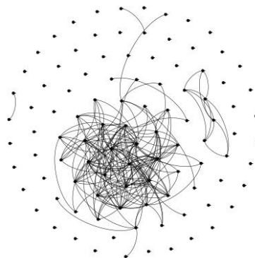
Fig. 5. The correlation network of stock returns based on \theta = 0.25
