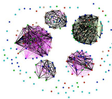
Fig. 3. Investors network clustering (Tomminello et al., 2012)
