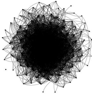
Fig. 4. The correlation network of stock returns based on 0.15
